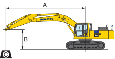
PC350-8M2 / PC350LC-8M2 A: Reach from swing center B: Arm top pin height C: Lifting capacity Cf: Rating over front Cs: Rating over side ⊗: Rating at maximum reach
